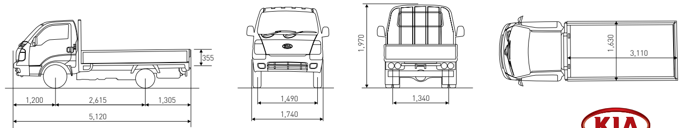
OPTIONAL FACTORY TRAY DIMENSIONS SHOWN
